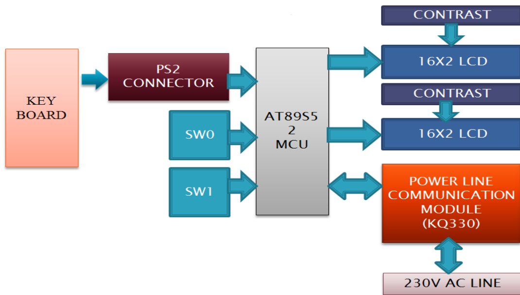
Figure.3. Block Diagram of Embedded Power Line Communication Transceiver Module (EPLCS)
