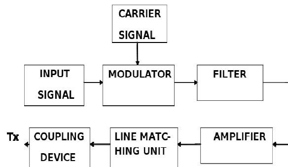
Figure.1. EPLCS TRANSMITTER
